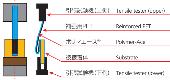
引張試験時概略図 Schematic diagram of tensile test
